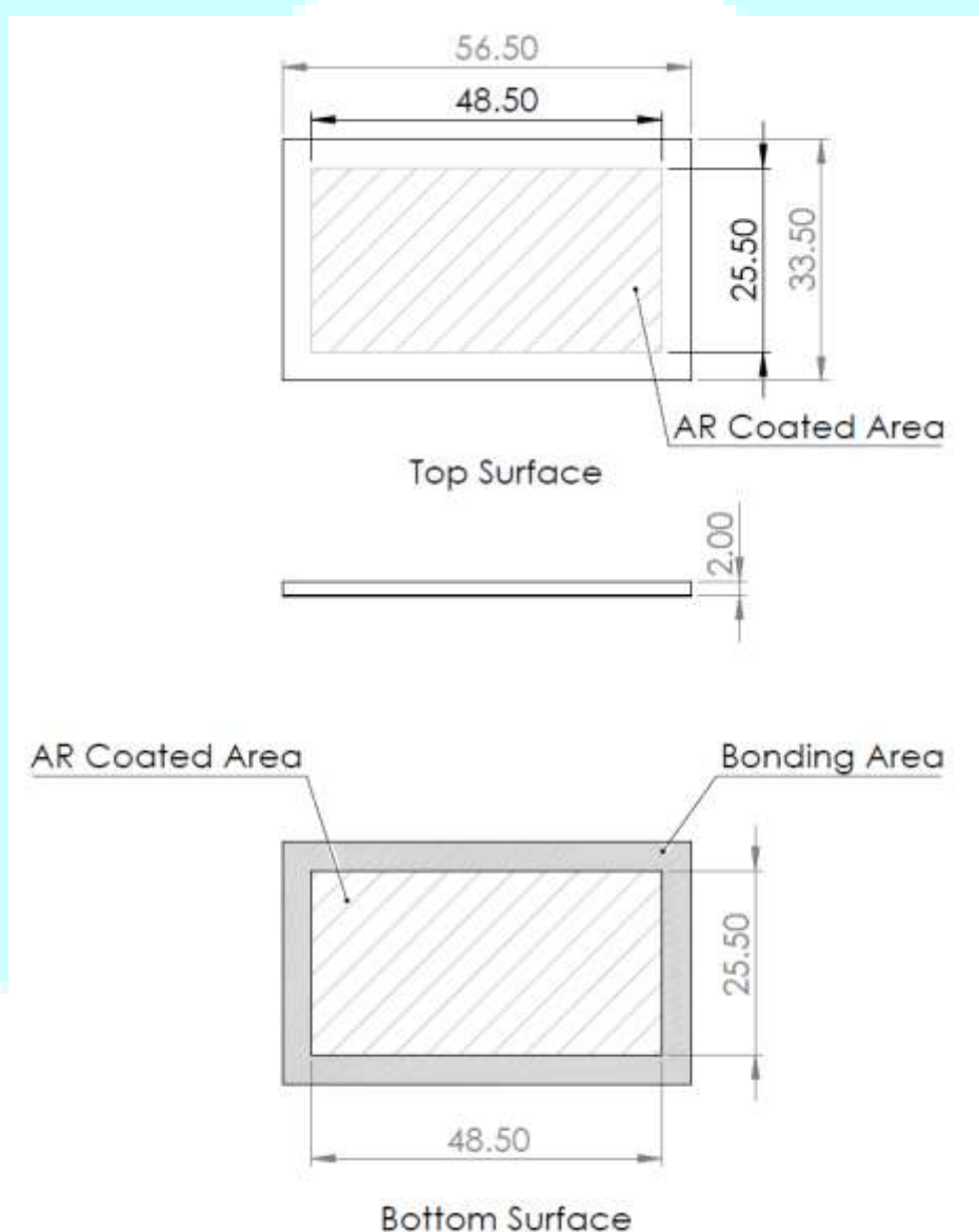
Figure 1: Schematic of the optical window for Imager-2
